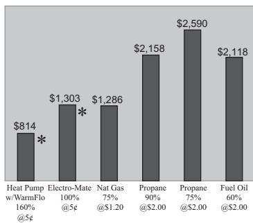
Annual Energy Cost Comparison 50,000 Btu/h, 8000 Degree Days
